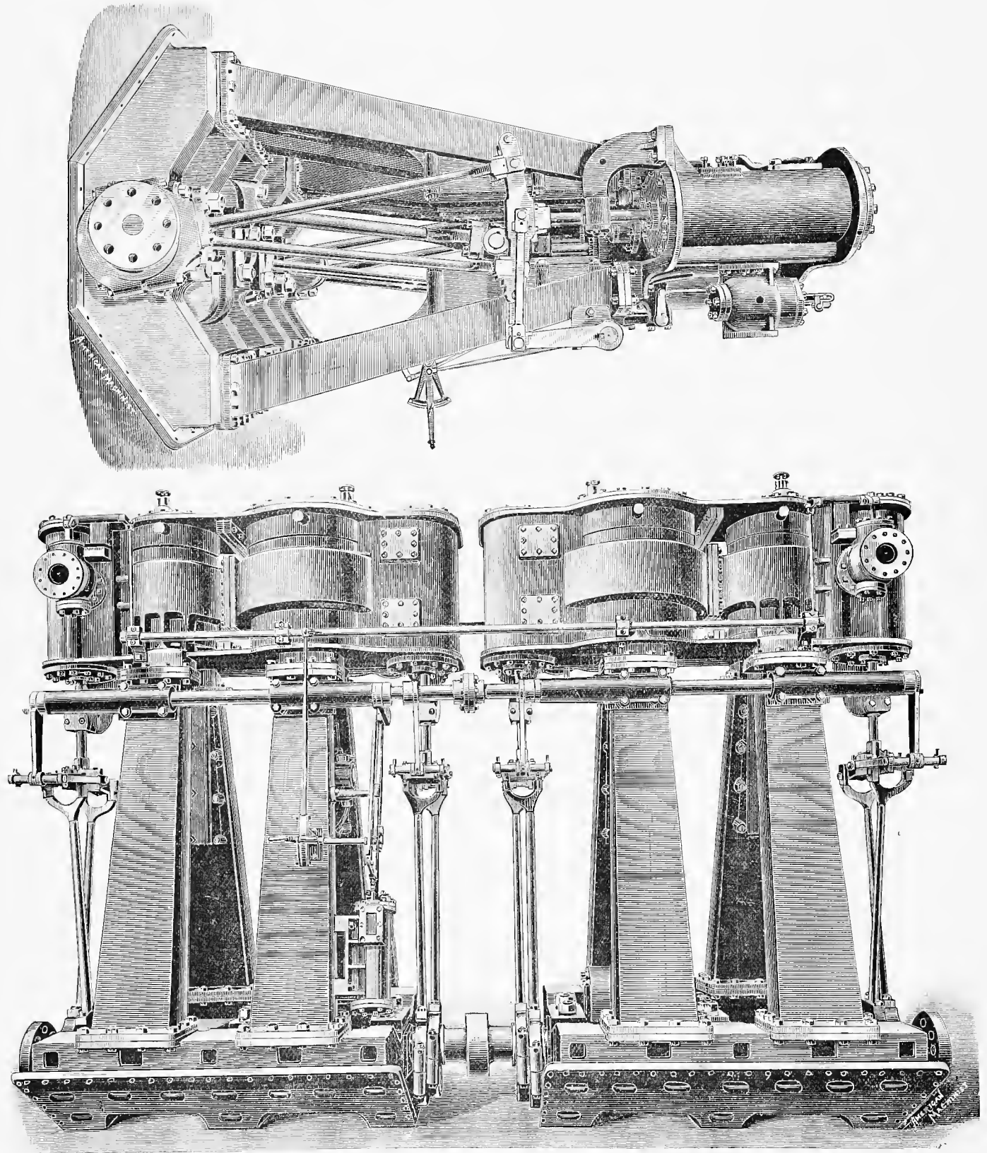
COMPOUND ENGINES OF HOBOKEN FERRYBOAT BREMEN.
